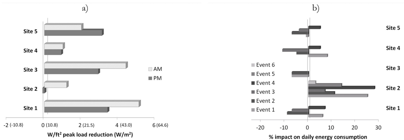
Figure 3 For all events, a) average peak load reductions, b) relative impact on daily energy consumption.
