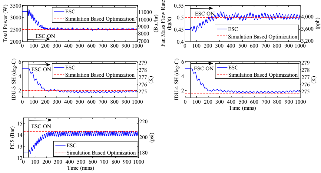
Figure 6. Input and output trajectories for multi-variable ESC control of 2H2C mode.
