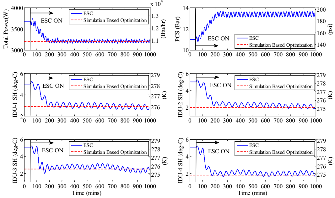
Figure. 4. Input and output trajectories for multi-variable ESC control of 4C mode.
