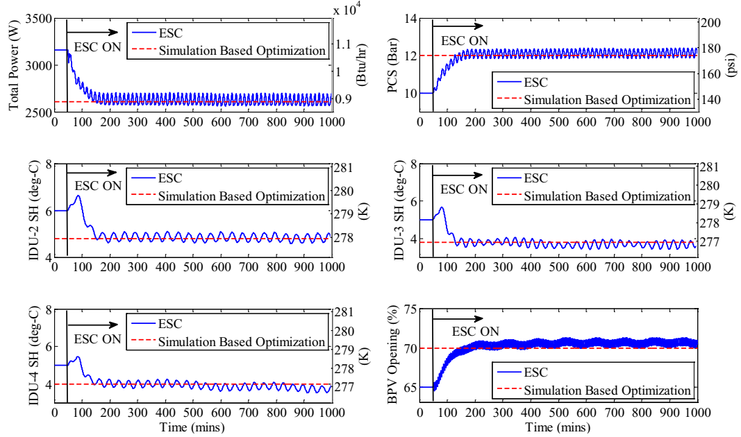
Figure. 5. Input and output trajectories for multi-variable ESC control of 1H3C mode.
