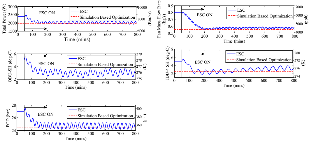
Figure. 7. Input and output trajectories for multi-variable ESC control of 3H1C mode.
