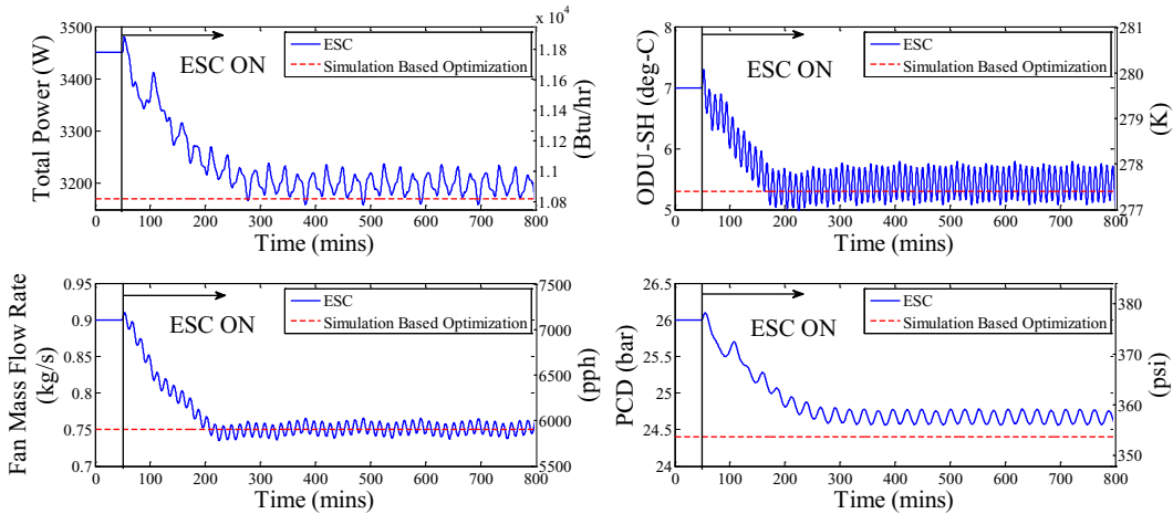
Figure 8. Input and output trajectories for multi-variable ESC control of 4H operation.
