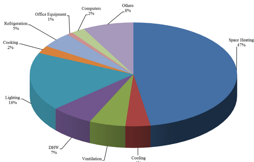
Figure 3-3a. Commercial building energy end-use estimates for heating-dominated climates (EIA 2003).
